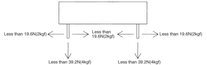
Fig.9.1 Stress onto the pins
