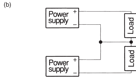
Fig.4.1 Series operation
