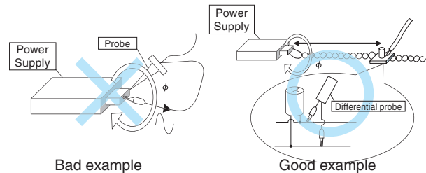
Fig.1.2 Example of measuring output ripple noise
