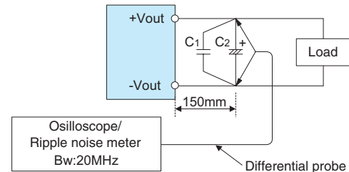
Fig.1.1 Measuring method of Ripple Noise
