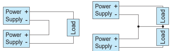
Fig.4.1 Examples of connecting in series operation
