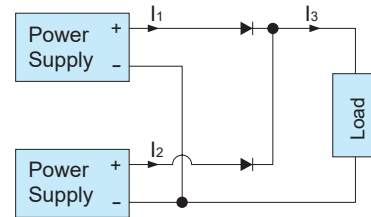
Fig.4.2 Example of redundancy operation
