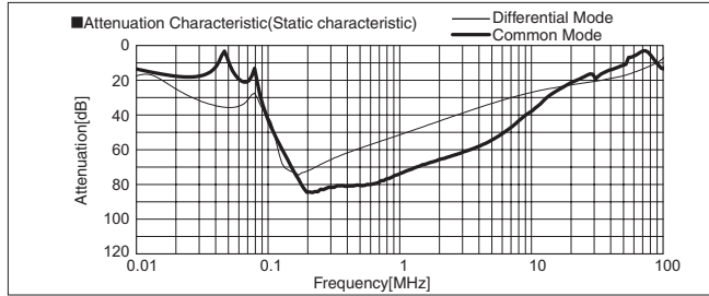
TSC-400-304-H/TSC-600-304-H
