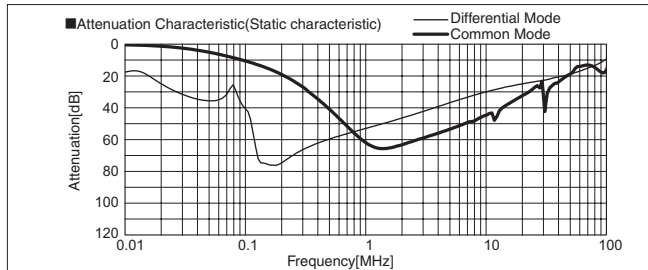
TSC-400-665-H/TSC-600-665-H
