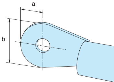
Fig.1.2 Terminals dimension
