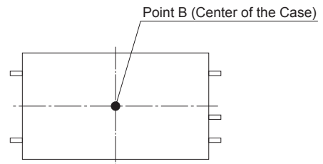
Fig.8.4 Temperature Measuring Point in the case of Forced Air Cooling (Upper Surface of the Case)
