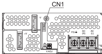
Fig.5.5 Front view of option -R (PJMA1000F)
