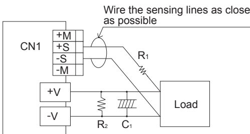
Fig.5.18 When using remote sensing function
