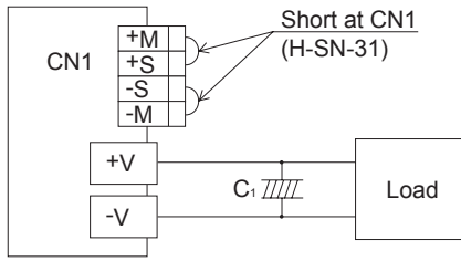
Fig.5.11 When not using remote sensing function
