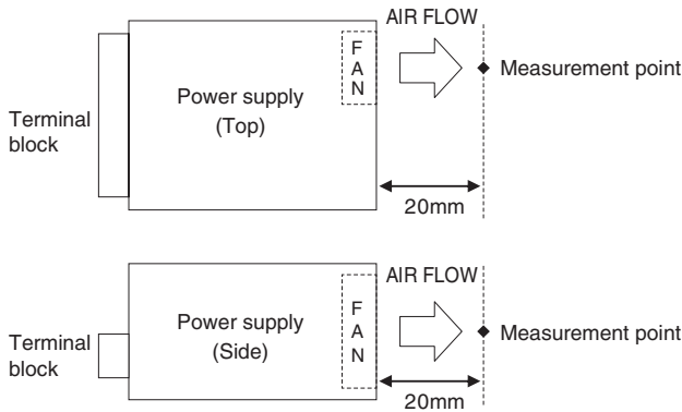
Fig.3.2 Temperature of measurement point for fan lifetime (PJMA600F)
