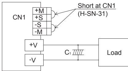
Fig.5.17 When not using remote sensing function
