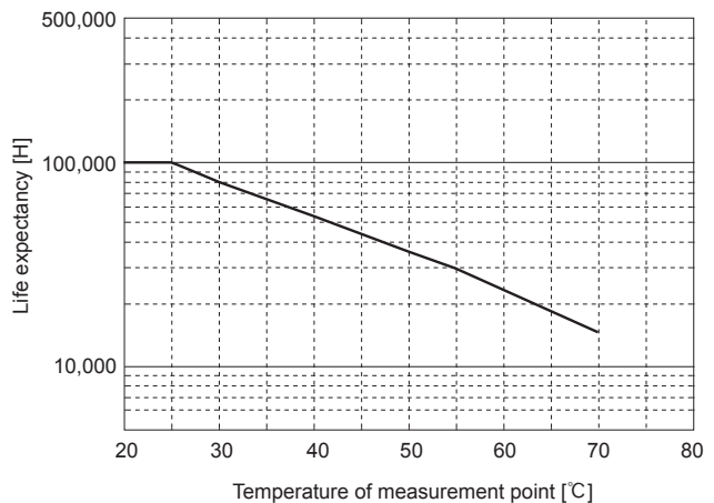
Fig.5.20 Life Expectancy of fan R(t)=90% (-F4)
