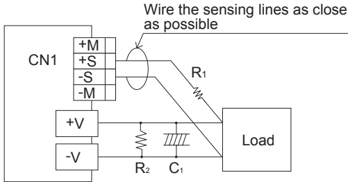
Fig.5.12 When using remote sensing function
