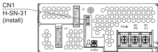
Fig.5.14 Front view of option -W1 (PJMA1000F)
