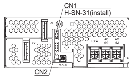
Fig.5.7 Front view of option -W (PJMA1000F)
