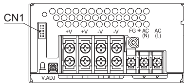
Fig.5.4 Front view of option -R (PJMA600F)
