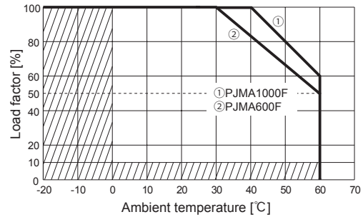
Fig.5.19 Ambient temperature derating curve (Option-F4)
