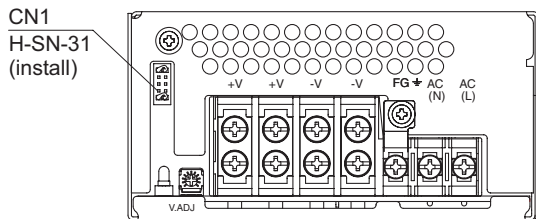
Fig.5.13 Front view of option -W1 (PJMA600F)
