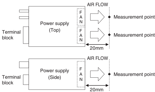
Fig.3.3 Temperature of measurement point for fan lifetime (PJMA1000F)
