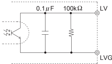
Fig.5.9 LV internal circuit
