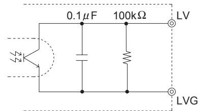
Fig.5.16 LV internal circuit
