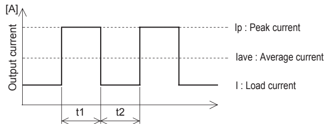
Fig.2.1 Peak current
