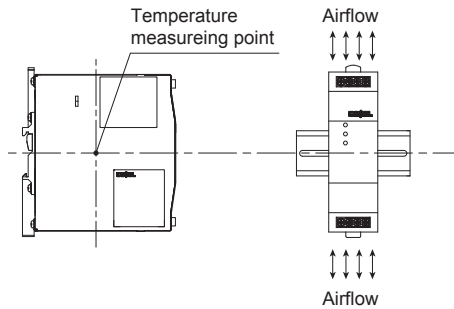
Fig.3.2 Temperature measurement point (Forced air)
