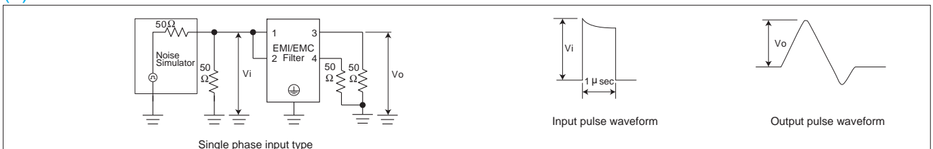
Fig.3.7 Pulse attenuation measurement diagram June 29, 2015
