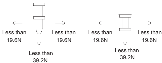
(option S) Fig.6.4 Stress onto the pins
