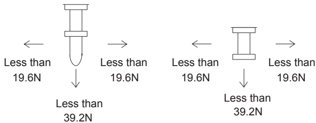
(option S) Fig.6.4 Stress onto the pins
