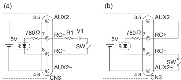
Fig 6.4 RC circuit example
