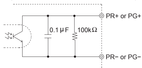
Fig 6.5 internal circuit of PR or PG
