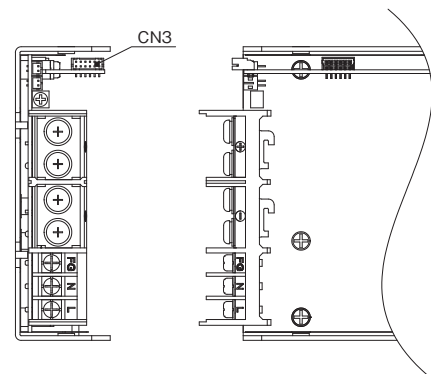
Fig 6.3 Example of option -R3 (AEA600F)
