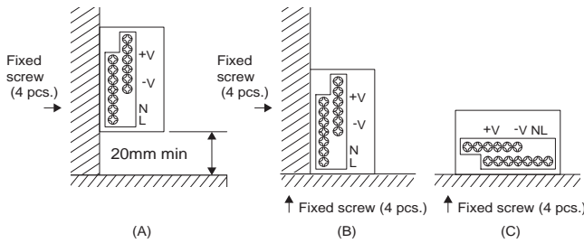
Fig.2.2 Installation method
