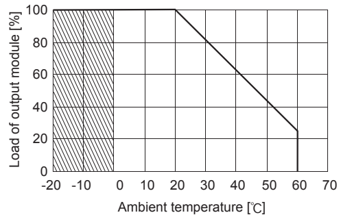
Fig. 6.4 Derating curve based on ambient temperature (-K)
