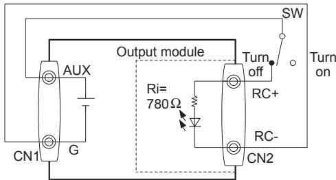
Fig. 3.3 Example of use with remote ON/OFF
