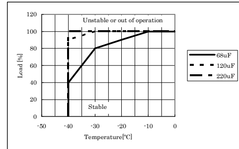
Load 0% to 100%(TUNS100)
