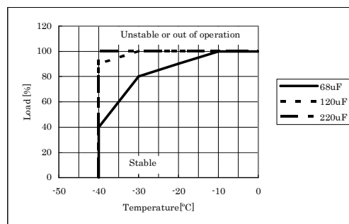
Load 0% to 100%(TUNS100)
