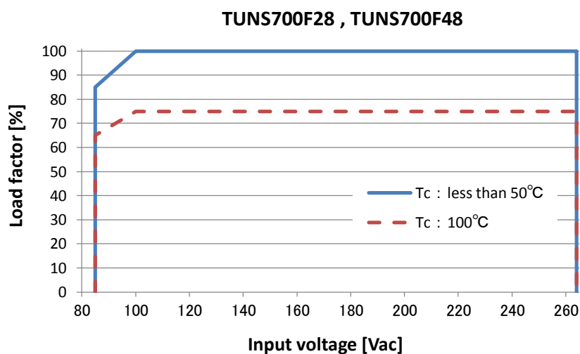
Fig.3.6 TUNS700F28/48 Output current and Input voltage derating
