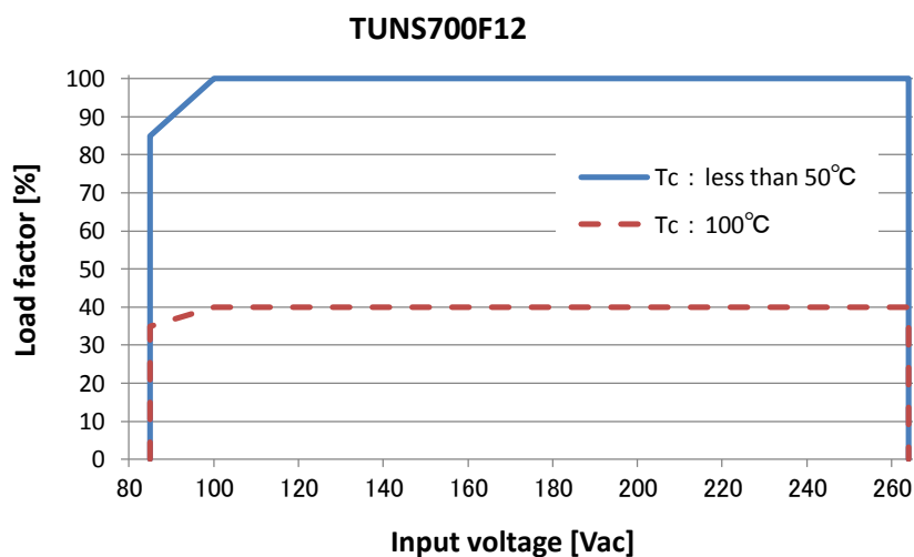
Fig.3.5 TUNS700F12 Output current and Input voltage derating
