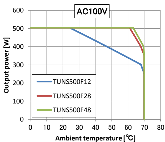
Fig.9.4 TUNS500F result
