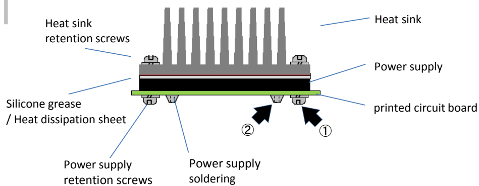
Fig.8.1 Mounting method
