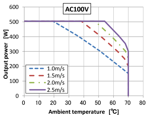
Fig.9.13 TUNS500F48 result
