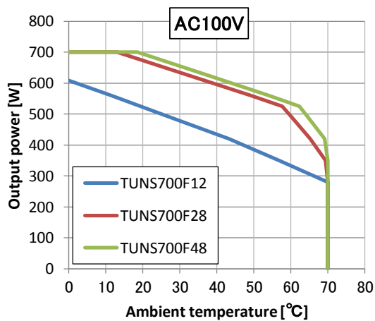
Fig.9.5 TUNS700F result
