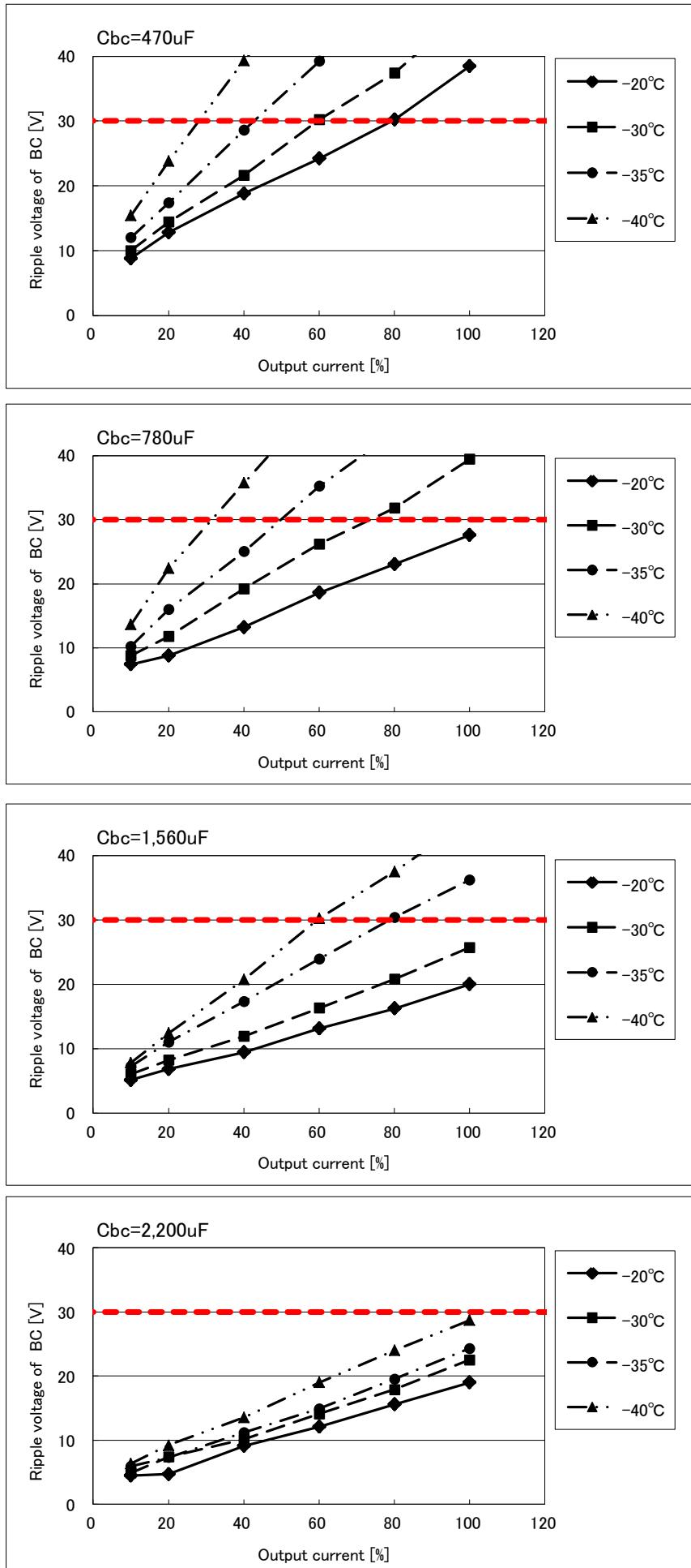
Fig.6.2 TUNS700F Relationship between ripple voltage of boost voltage and temperature ( V_{in}=AC85V )
