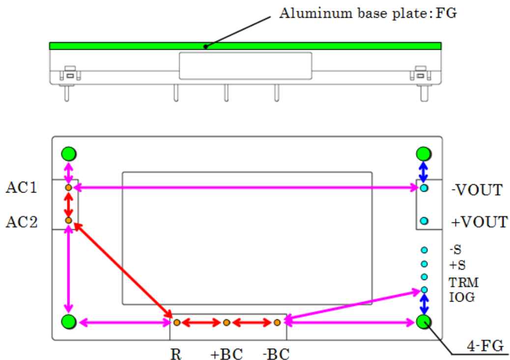
Fig.10.1 Insulation distance
