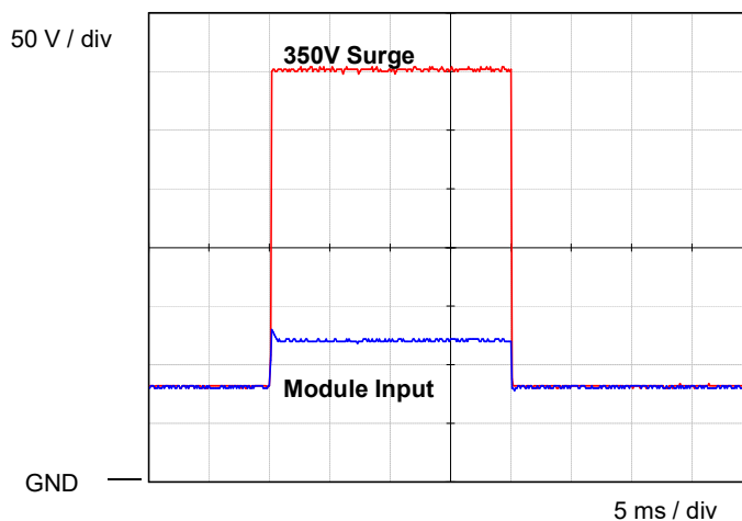
Fig.5.2 Clamped surge voltage
