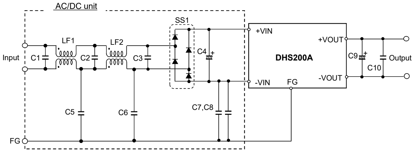
Fig.1 testing circuitry (from No.1 to No.5, No.7)
